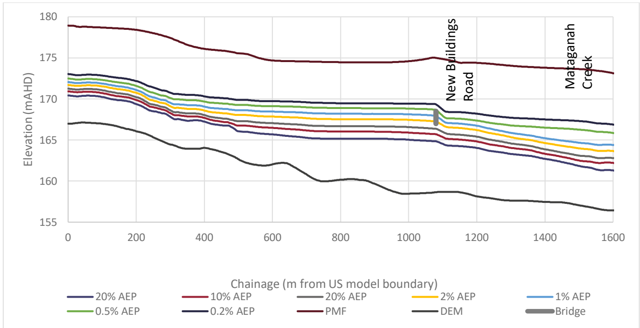
Figure 6-5 New Buildings Long Section
