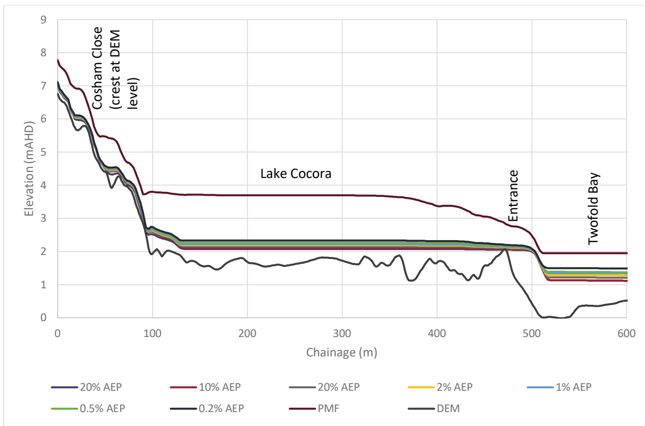
Figure 6-17 Lake Cocora Long Section
