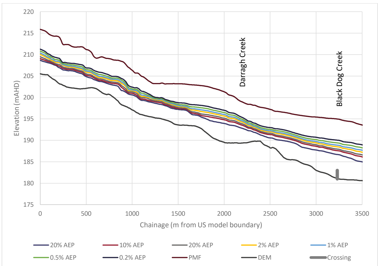
Figure 6-3 Rocky Hall Long Section
