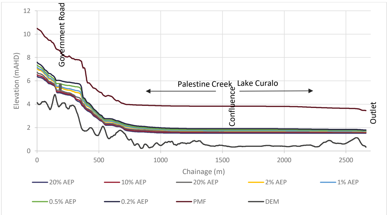
Figure 6-15 Lake Curalo Long Section
