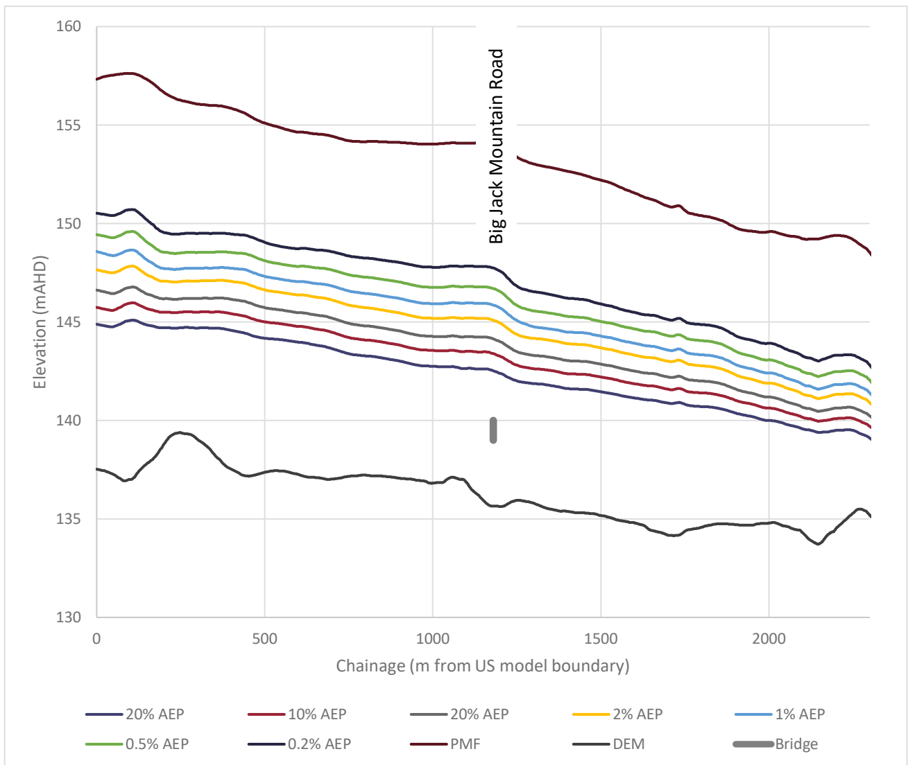
Figure 6-7 Burragate Long Section
