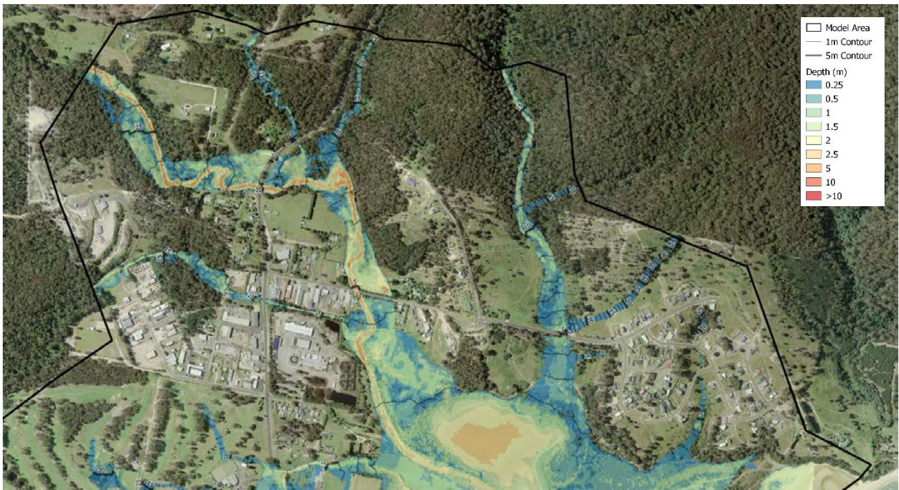
Figure 6-11 Lake Curalo Northern Tributaries (with 1% AEP flooding)
