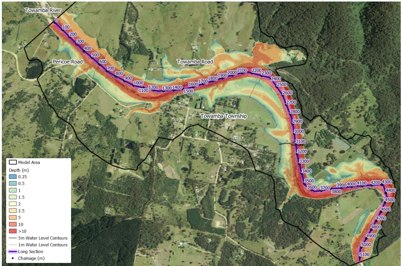
Figure 6-10 Towamba Flooding and Long Section Chainage (with 1% AEP flooding)
