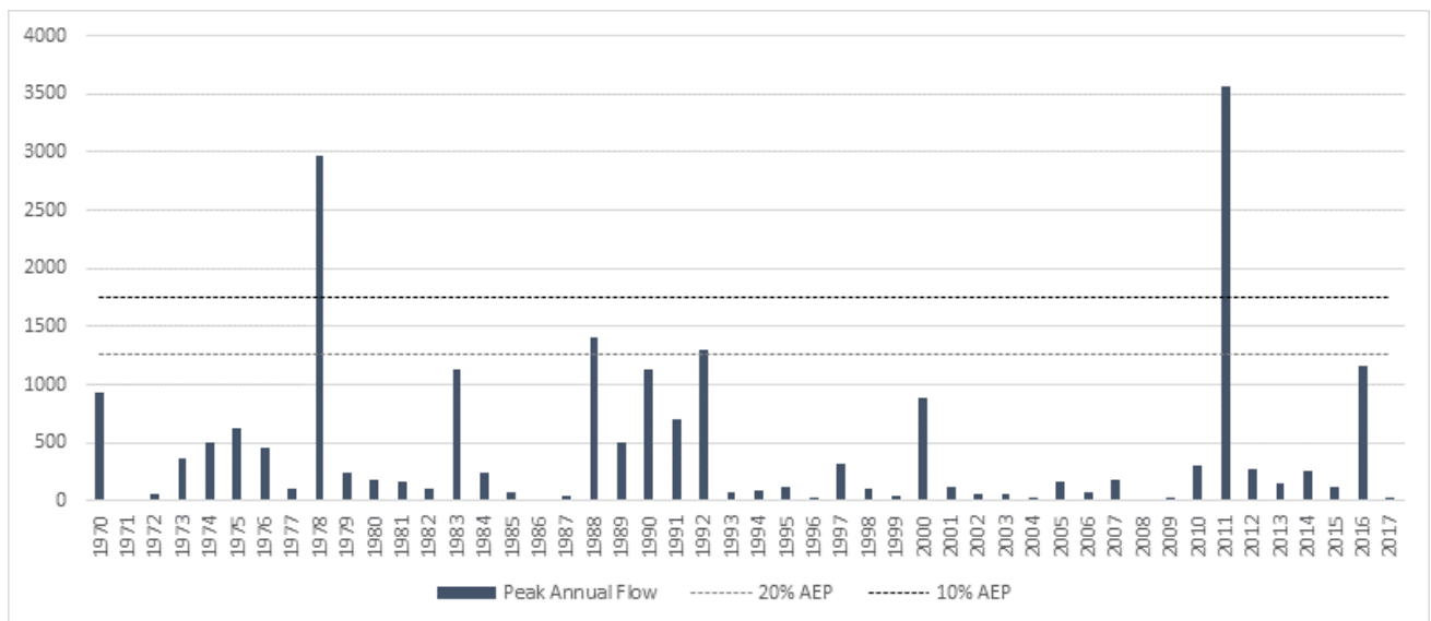
Figure D-8 Towamba Annual Peak Flow
