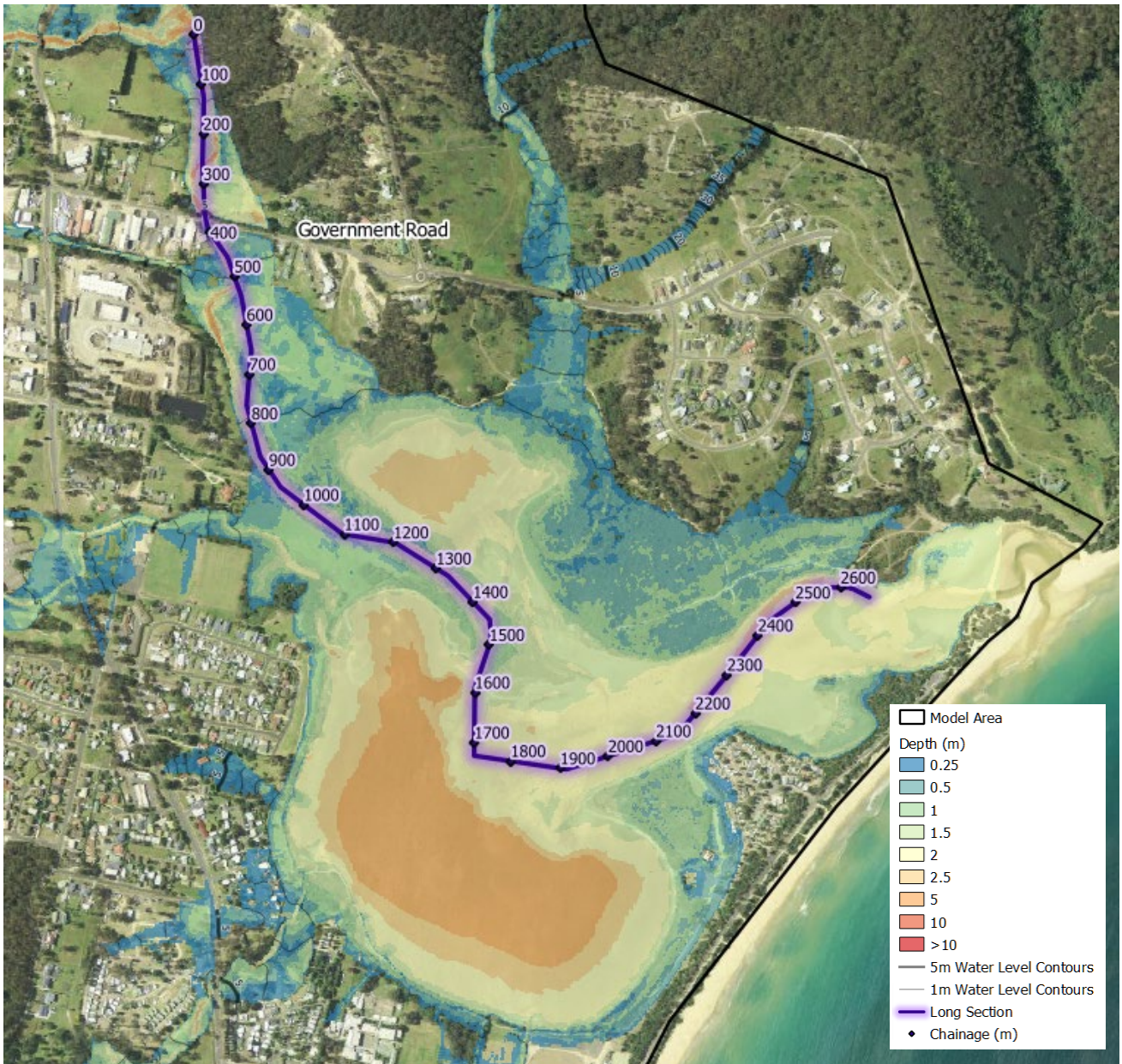
Figure 6-14 Lake Curalo Flooding and Long Section (with 1% AEP flooding)
