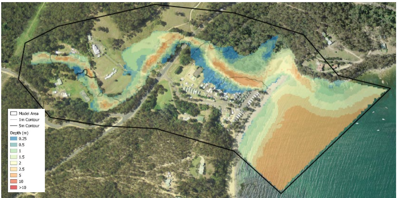
Figure 6-18 Shadrachs 1% AEP Flooding
