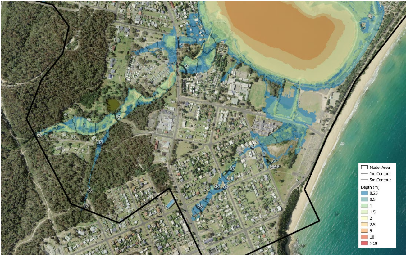
Figure 6-13 Lake Curalo Southern Tributaries (with 1% AEP flooding)
