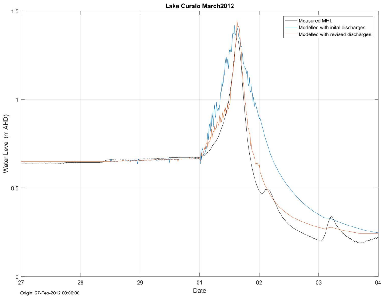
Figure D-3 Comparison of modelled lake water levels with the measured water levels from the MHL gauge within Lake Curralo for the March 2012 breakout event.
