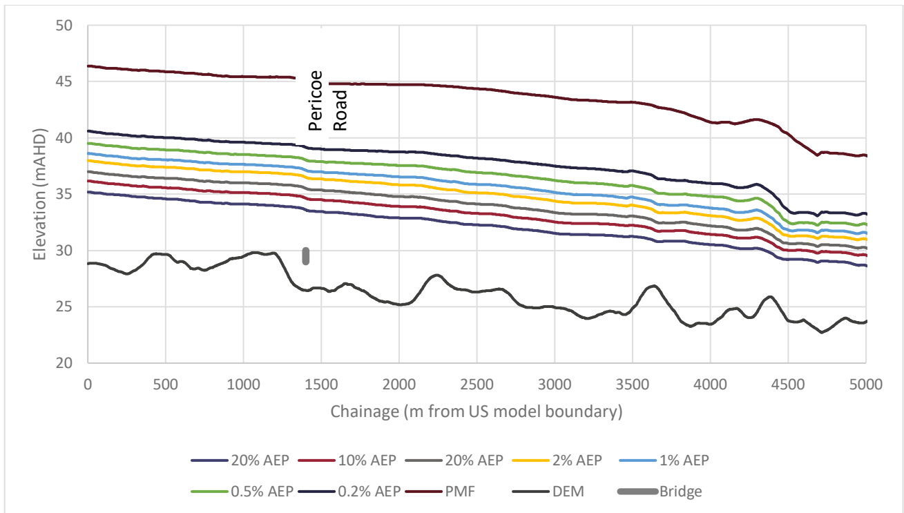
Figure 6-9 Towamba Long Section
