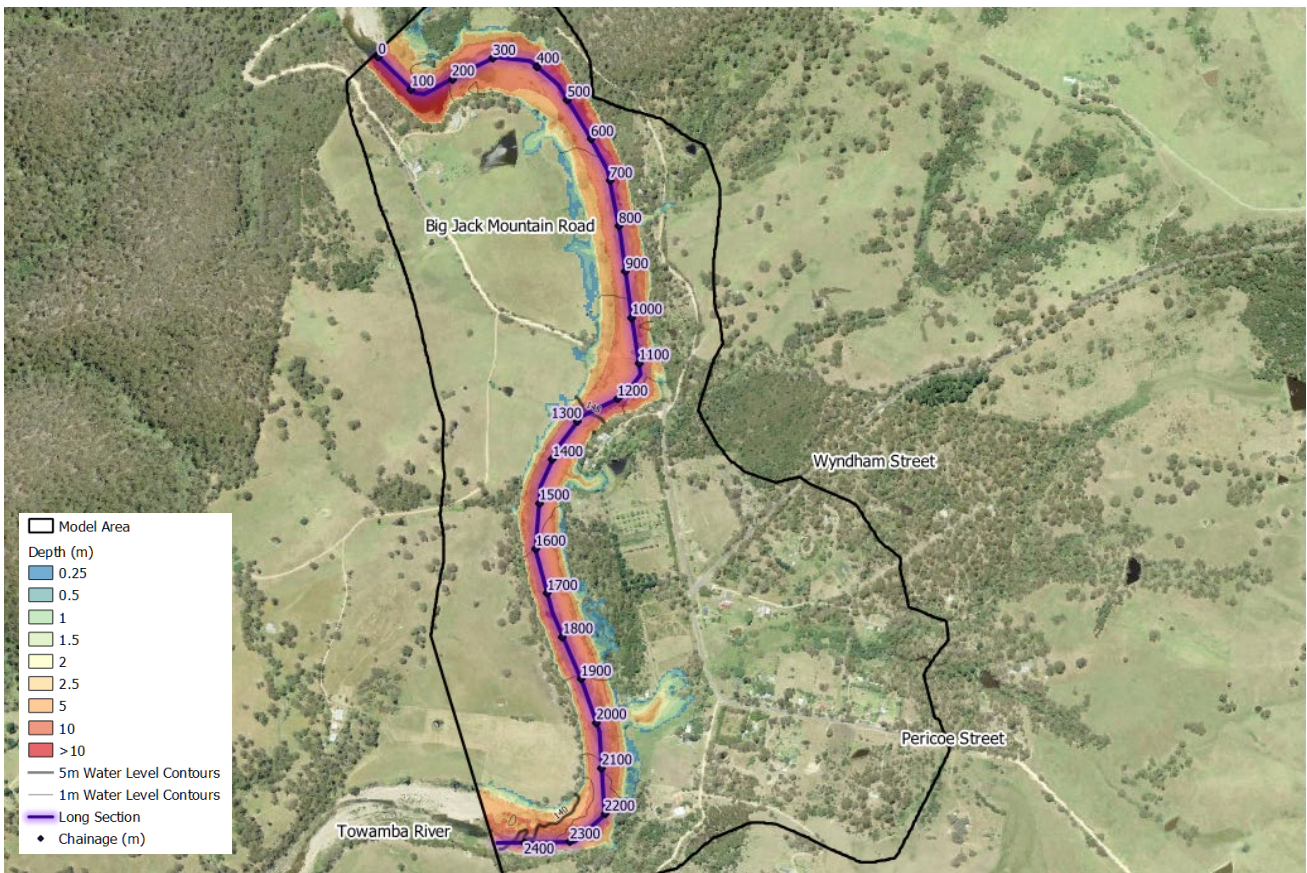
Figure 6-8 Burragate Flooding and Long Section Chainage (with 1% AEP flooding)
