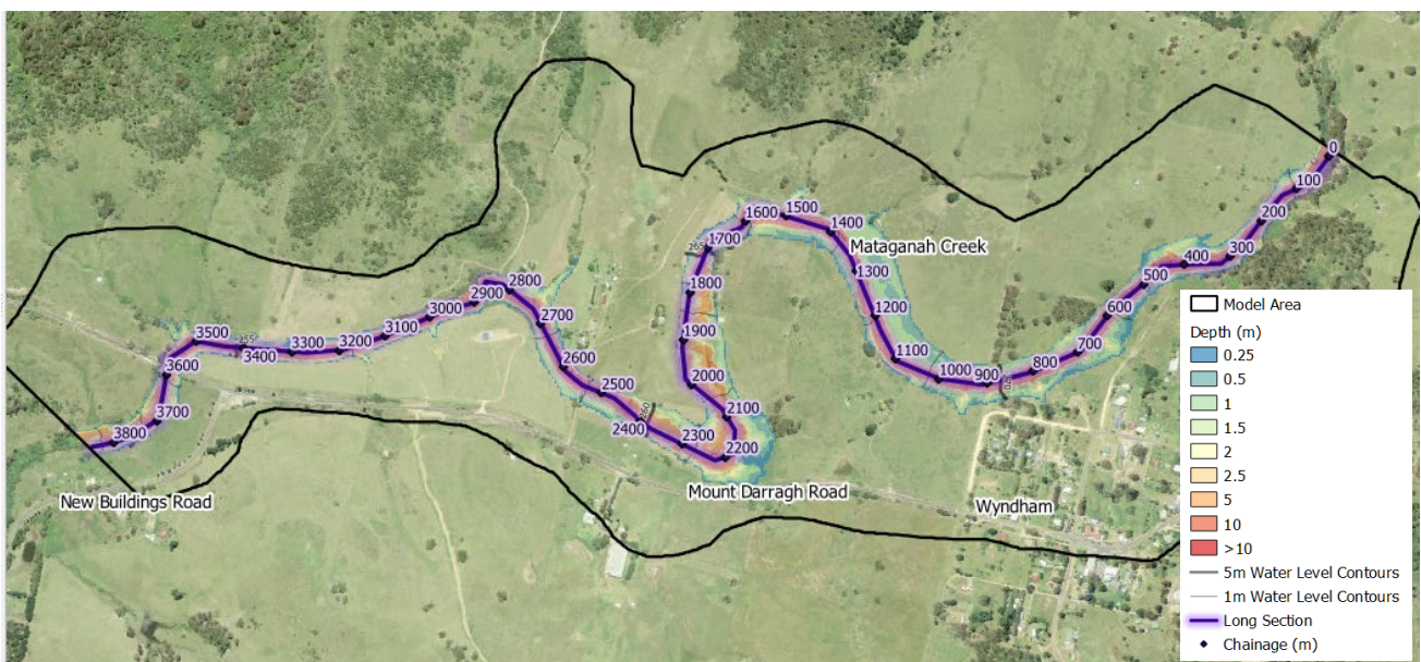
Figure 6-2 Wyndham Flooding and Long Section Chainage (with 1% AEP flooding)
