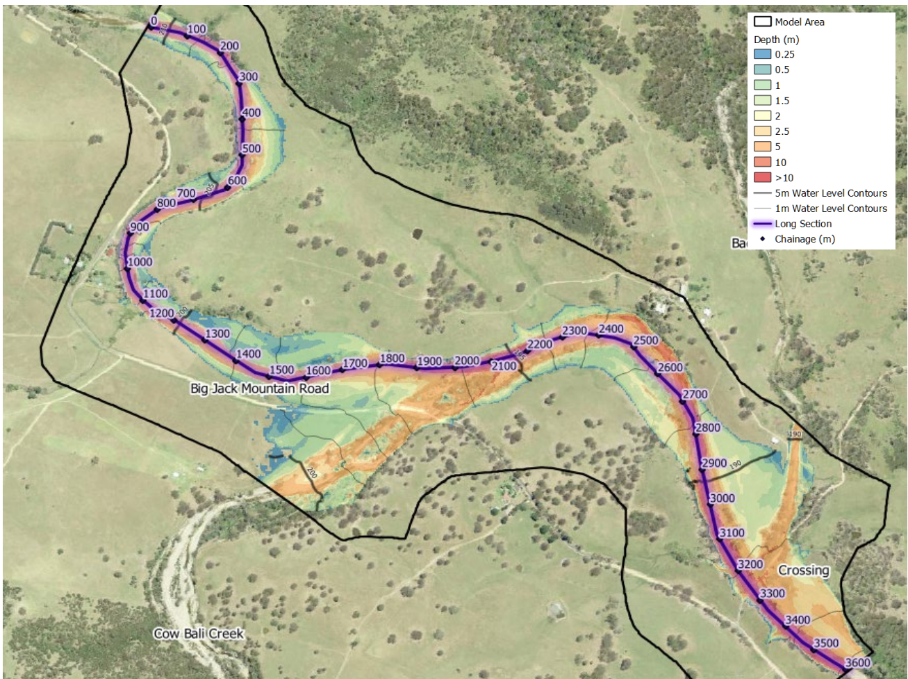
Figure 6-4 Rocky Hall Flooding and Long Section Chainage (with 1% AEP flooding)
