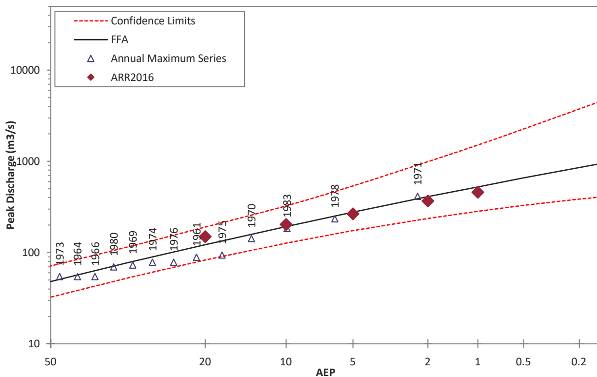
Figure D-5 Rocky Hall FFA Comparison
