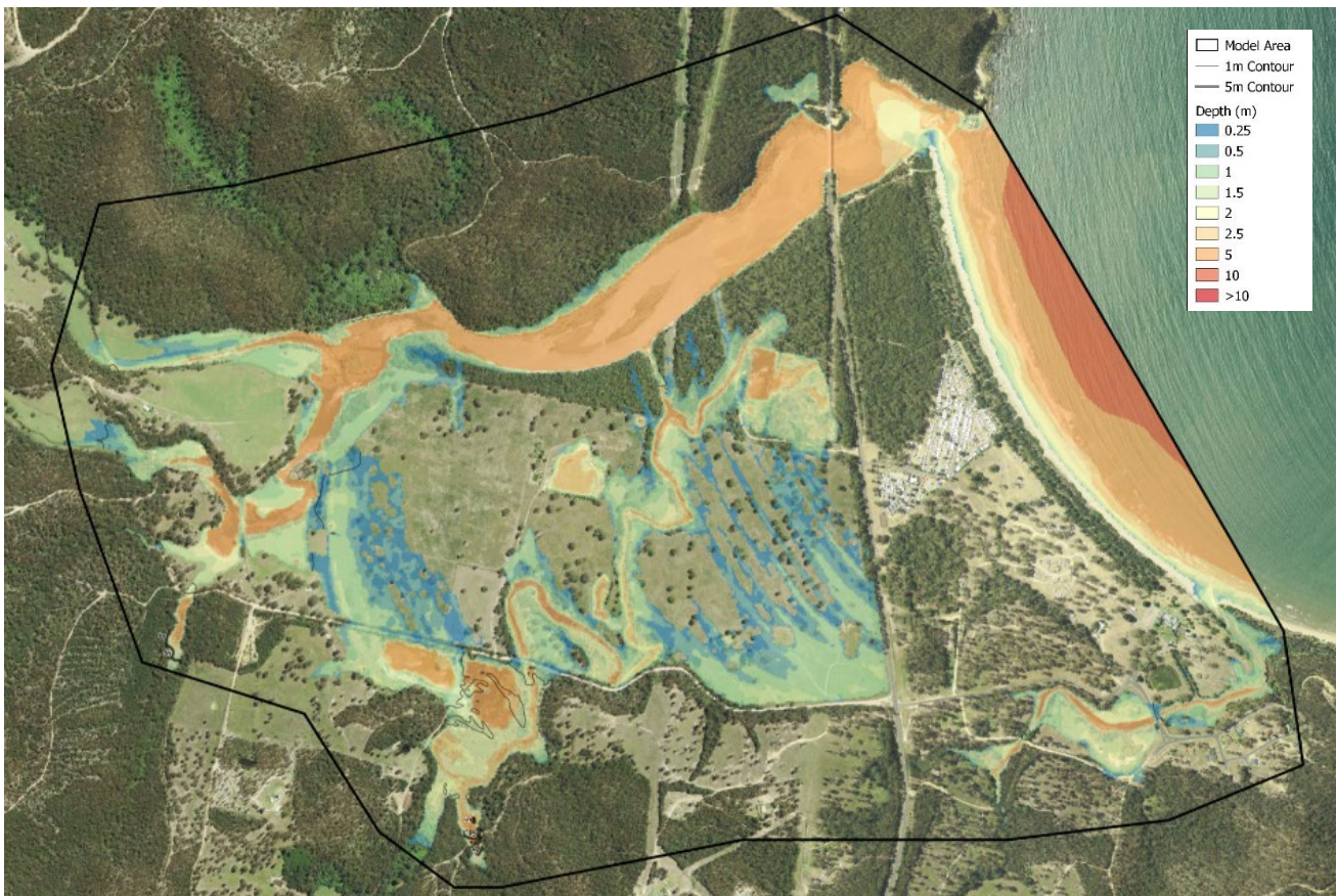
Figure 6-19 Nullica Boydtown 1% AEP Flooding
