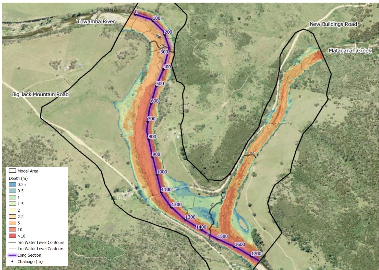
Figure 6-6 New Buildings Flooding and Long Section Chainage (with 1% AEP flooding)
