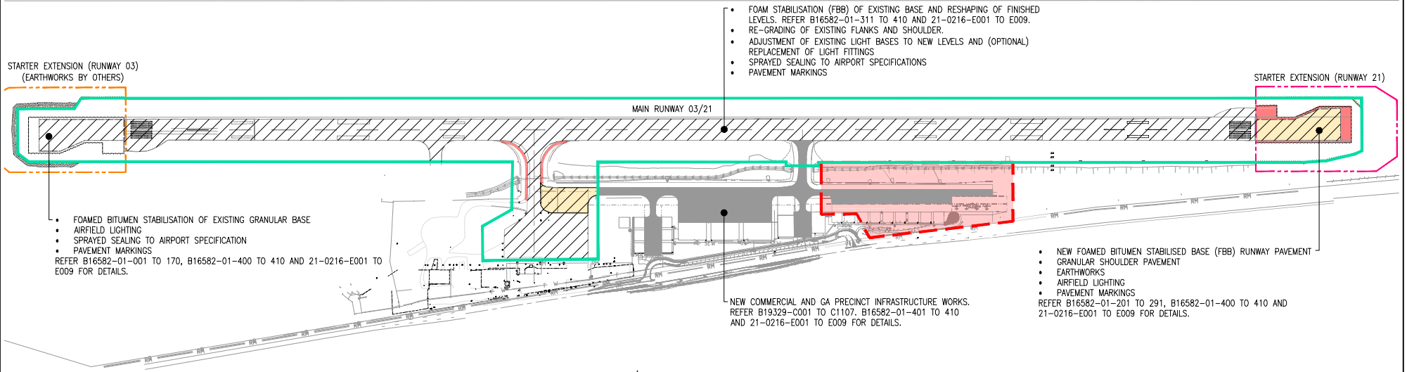
MAIN RUNWAY 03/21 INFRASTRUCTURE WORKS LAYOUT PLAN SCALE: 1:2500
