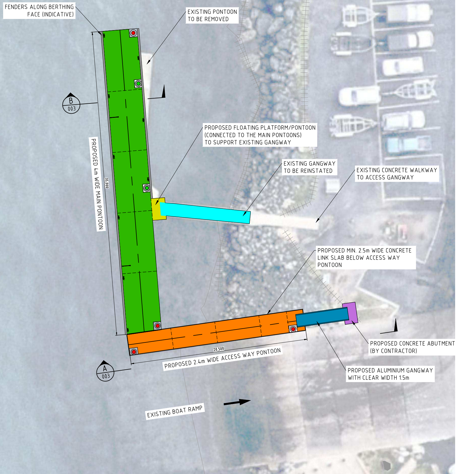
GENERAL LAYOUT PLAN SCALE 1:125
